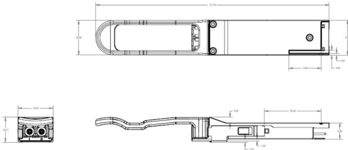
Figure 2 – MTL4E1Q mechanical drawing
