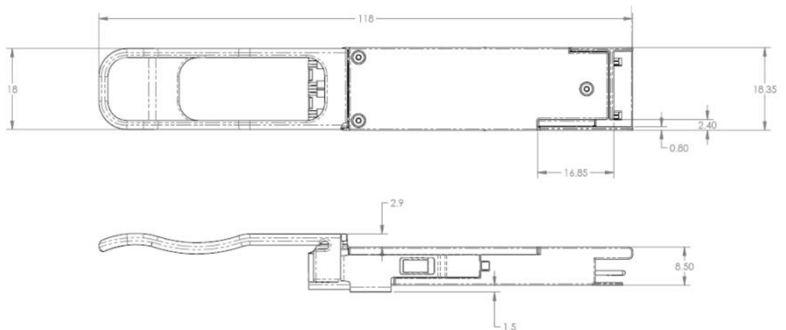
Figure 2 – MTL4P1QM1C mechanical drawing
