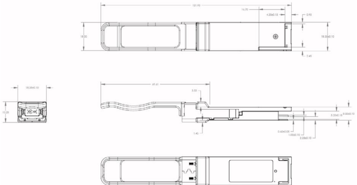
Figure 3 – MTL410QD2C mechanical drawing
