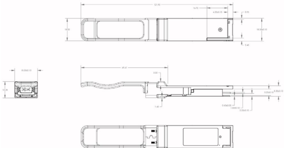
Figure 3 – MTL410QE2C mechanical drawing
